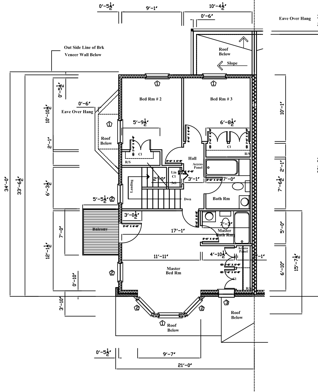
Second Floor Plan - Unit "A"
