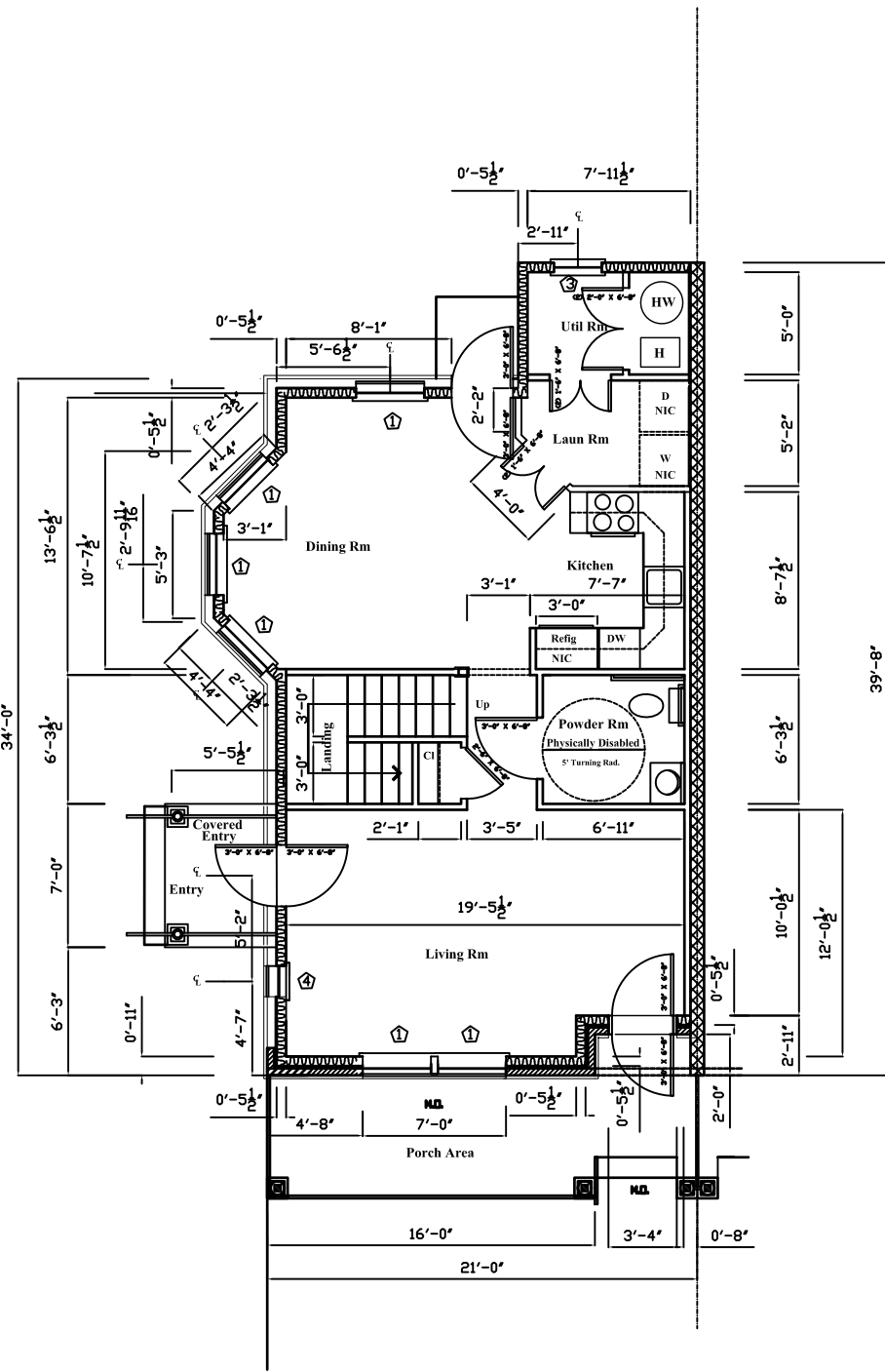
First Floor Plan - Unit "A"
